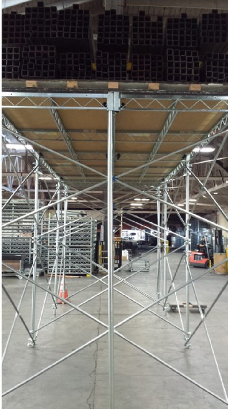
Figure 3-3 Load Step 1, Platform loaded to 202.76 lbs/ft 2
