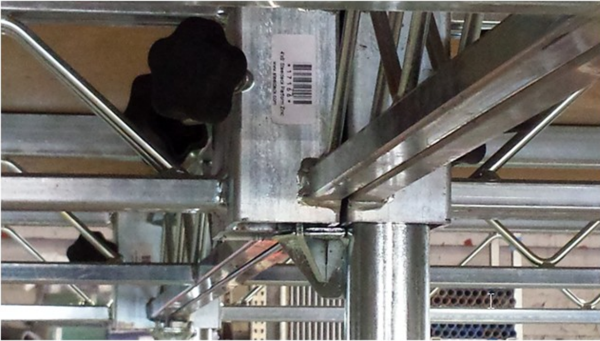
Figure 3-7 No distress of critical leg-to-deck support mount
